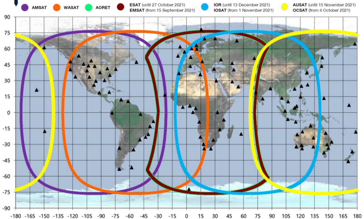
Figure 1: Fugro Global Beams and Reference Sites (source: Fugro )
