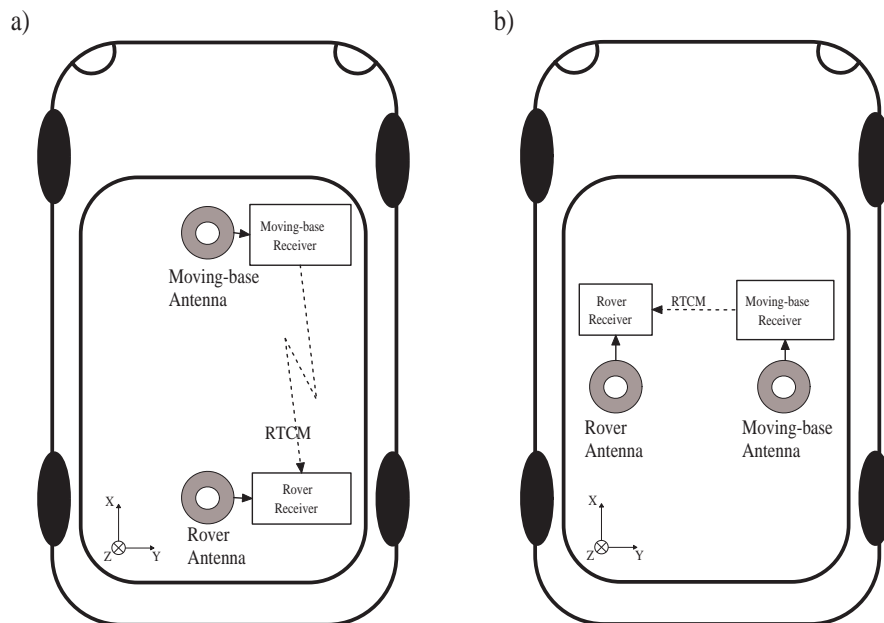
Figure 1-2: Moving-base attitude determination setup. a) default configuration. b) example of non-default configuration.
